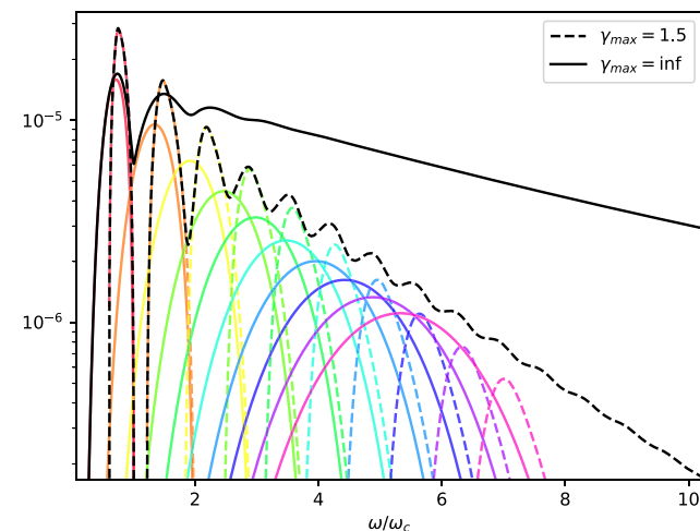
FIG. 1. The total plasma emission coefficient j_{\omega} for \theta = 0.45\pi calculated for 300 harmonics as a function of \omega/\omega_c for \gamma_{\max} = 1.5 (black dashed line) and without cutoff (black solid line) together with their first 10 harmonics (color solid and dashed lines).
